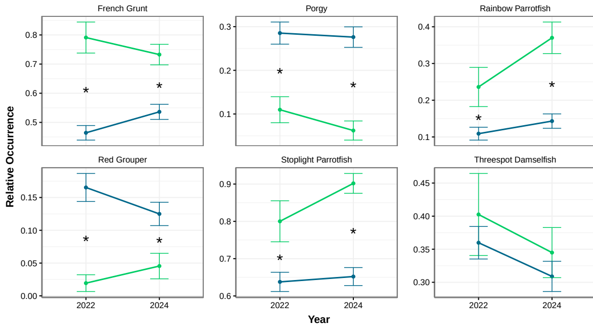
Survey Location — M:IR — Outside Relative occurrence \pm standard error is shown within the M:IR reef sites (M:IR, green) and outside the restoration areas in the Florida Keys (outside, blue). Significant differences between M:IR and open densities are denoted with an asterisk (*) within each survey year.
